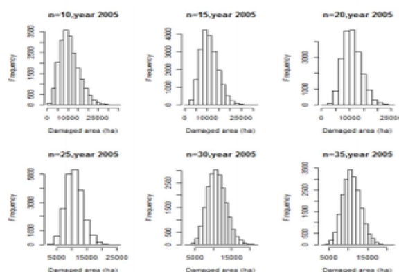
Figure 1. An example of the frequency distribution of 20,000 estimates of the total damage caused by sudden aspen decline (SAD) of SRS design and selected sample sizes. The x-axis is area damaged (ha), the y-axis is frequency
