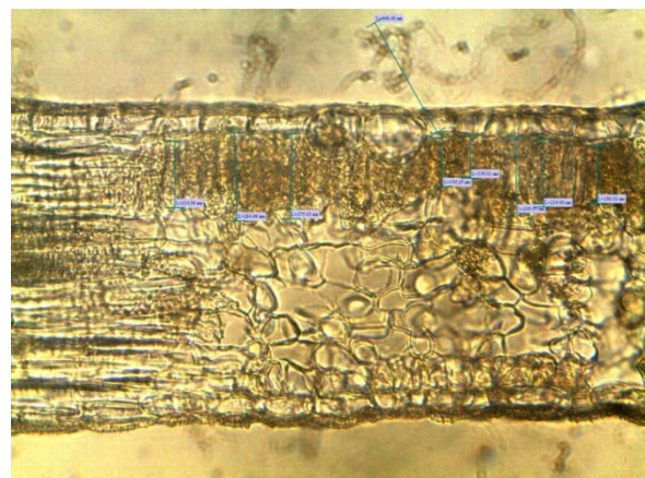
Figure 03. Cross section of the regenerated Castanopsis boisii leaf
