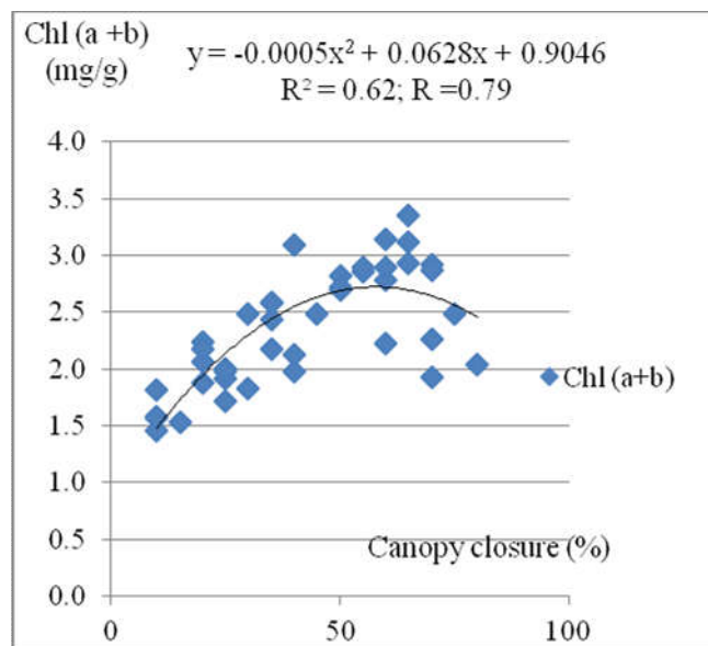
Figure 07. Relationship between canopy closure and total chlorophyll(a+b)
