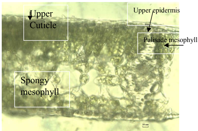
Figure 02. Cross section of Castanopsis boisii leaf
