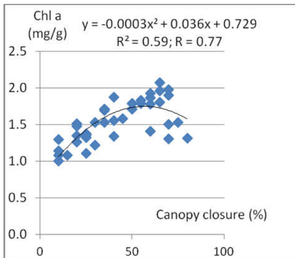
Figure 04. Relationship between canopy closure and chlorophyll a content
