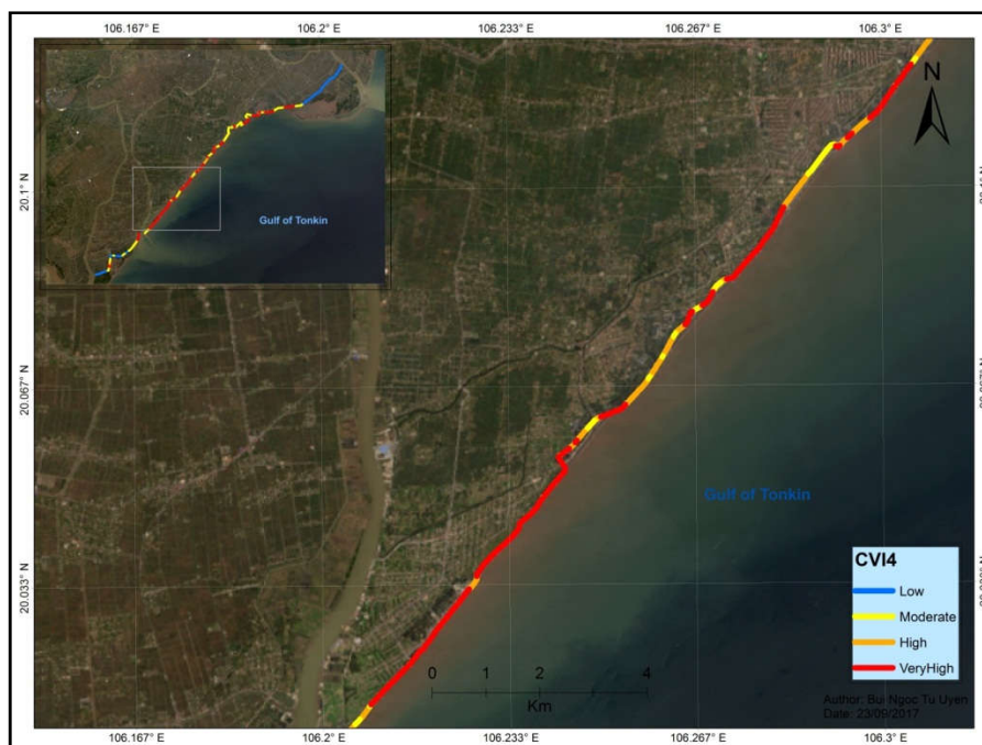
Figure 4. Coastal vulnerability from Hai Ly to Thinh Long communes
